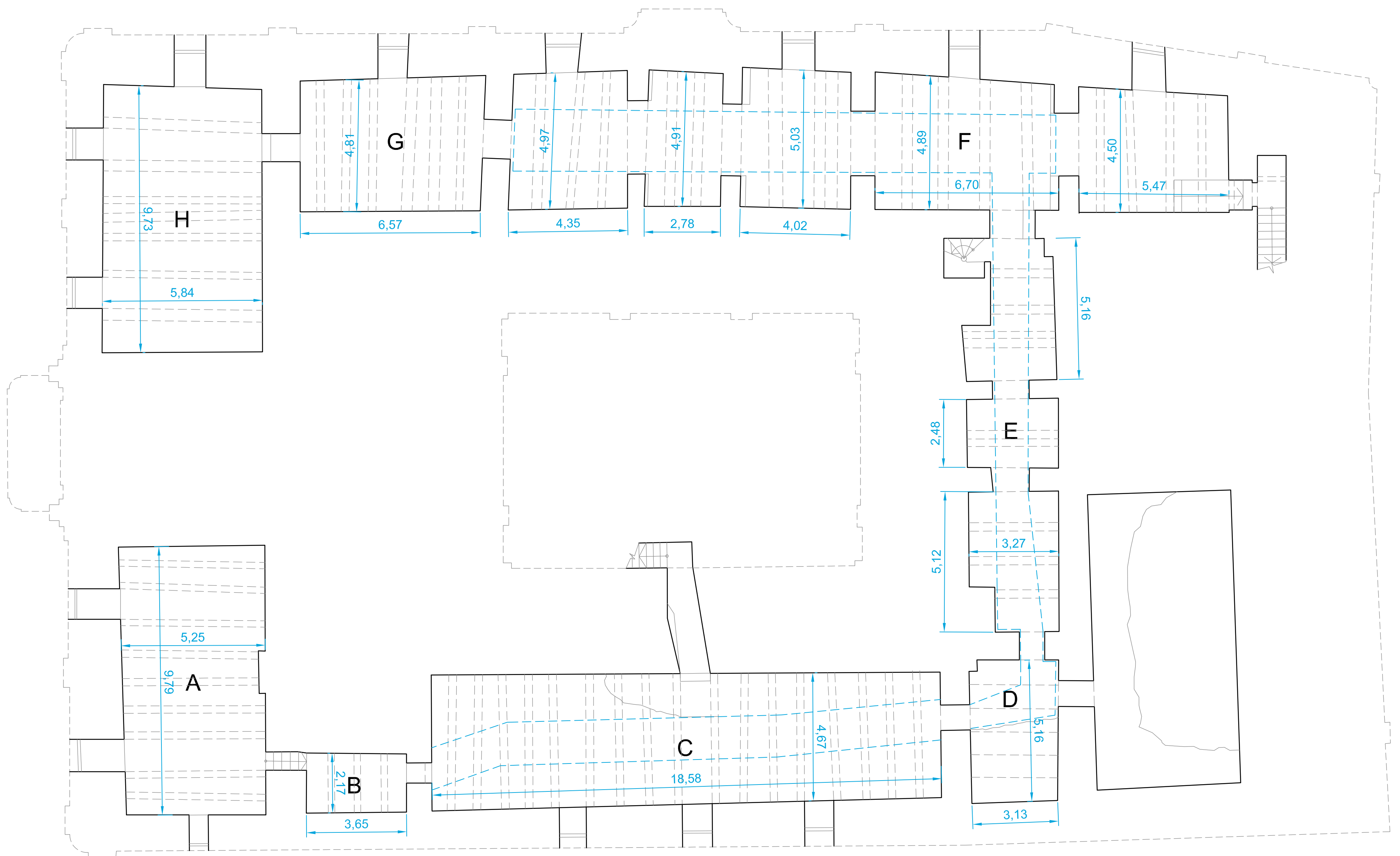
BASEMENT LEVEL PLAN --- Perimeter of timber walkways (indicative only) Scale 1:100
